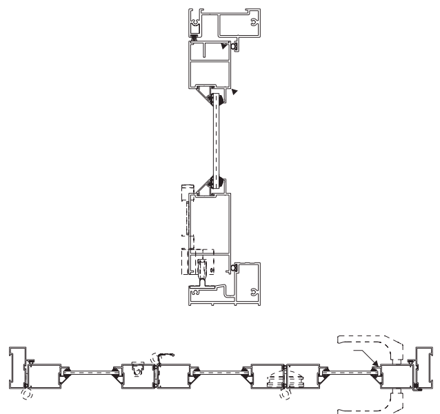
Assembly Diagram
